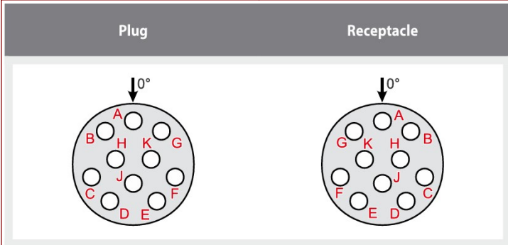
Layout of pins – plug and receptacle
