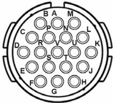
Layout of pins – connector side view
